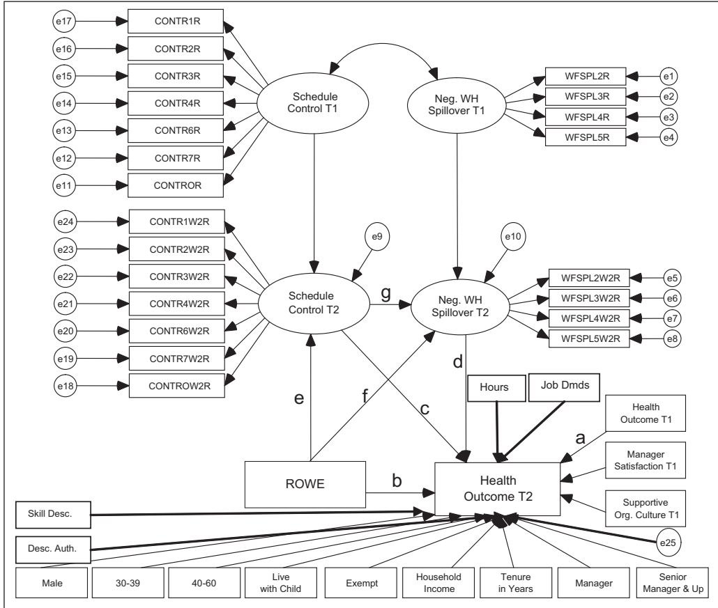
Figure 1. Conceptual Structural Equation Model
